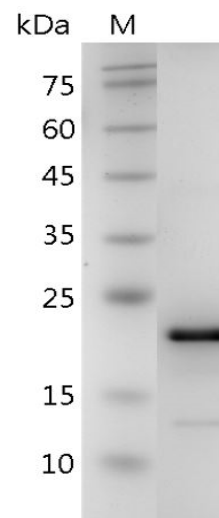
SDS-PAGE analysis of recombinant human FGF-12
